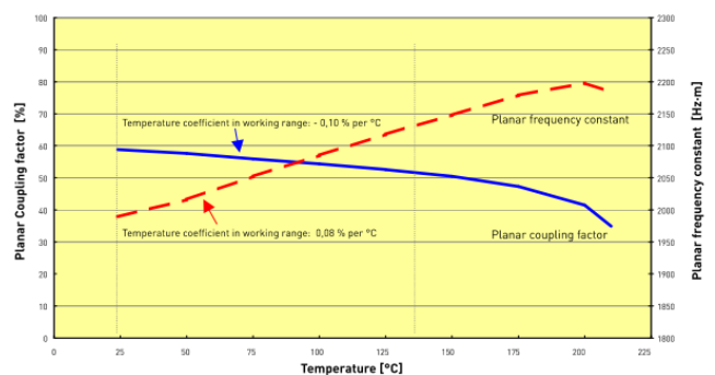
Planar coupling factor (blue) and planar frequency constant (red) for Ferropem Pz21 as a function of temperature. Very linear and stable behaviour is observed within the recommended working temperature range between 20°C and 130°C.
