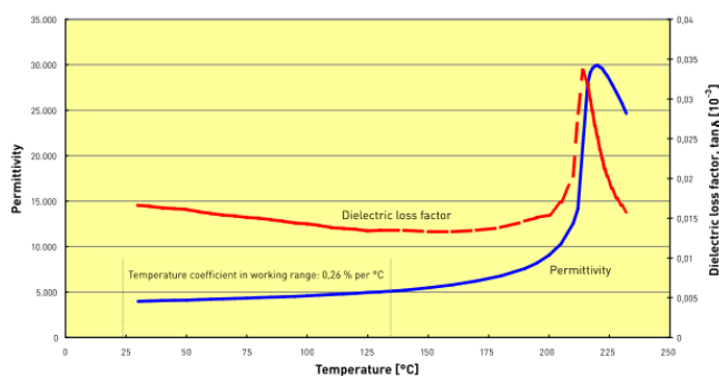
Permittivity (blue) and dielectric loss factor (red) for Ferropem Pz21. The Curie point is above 220°C and the increase in permittivity in the recommended working range from 20° to 130°C is only 0.26% per °C
